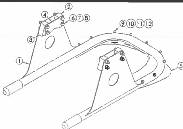
Figure 1. Nose Gear Gravel Deflector Parts
