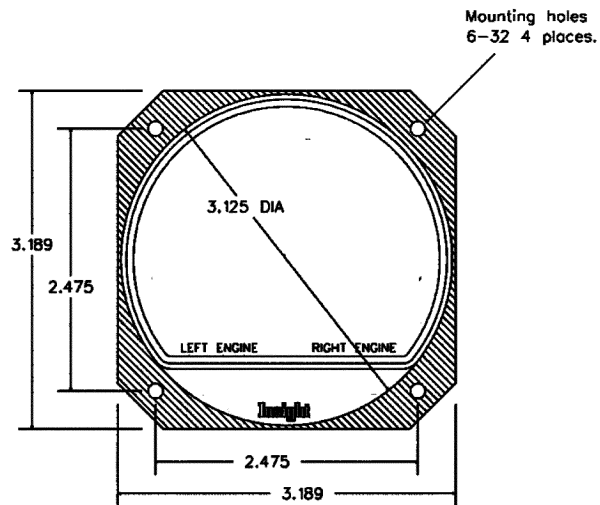
INSTRUMENT BEZEL AND PANEL HOLE LAYOUT
