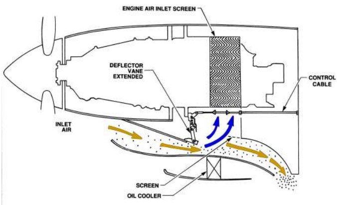
Figure 3-12. Turboprop sand and ice separator (inertial).
