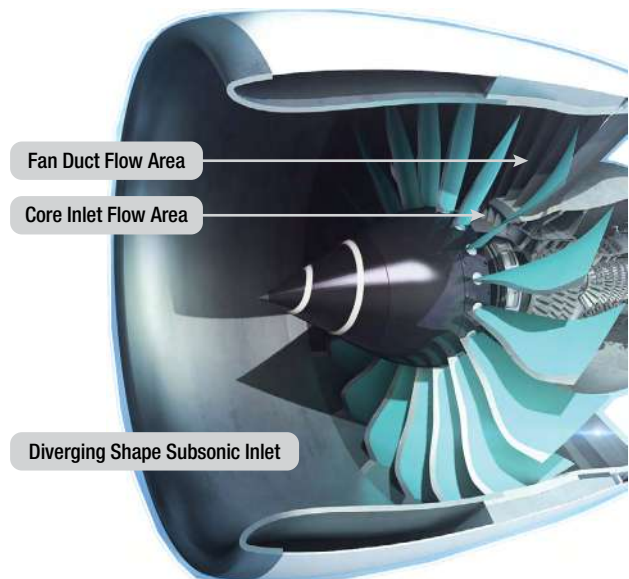
Figure 3-4. Diverging inlet for ultra-high-bypass turbofan.
