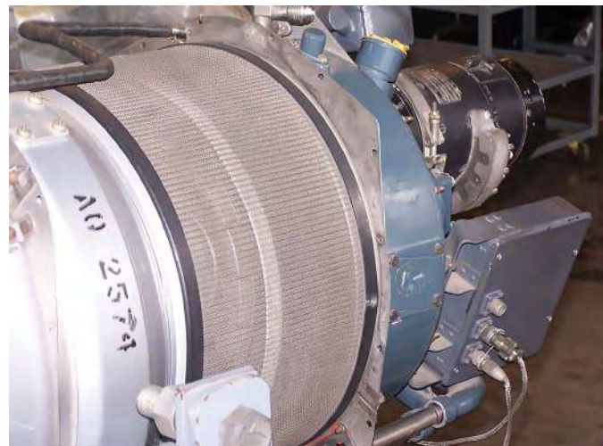
Figure 3-16. Example of a turboprop engine that incorporates inlet screens.
