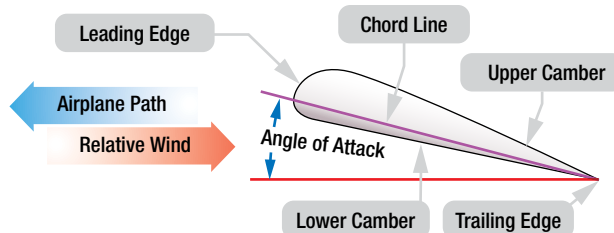
Figure 2-8. Wing terminology.
