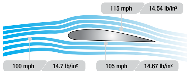
Figure 2-9. Airflow over a wing section.
