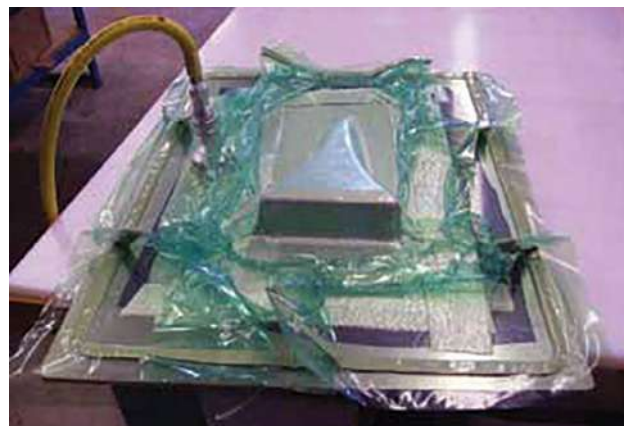
Figure 3-38. Vacuum bagging of contoured part.
