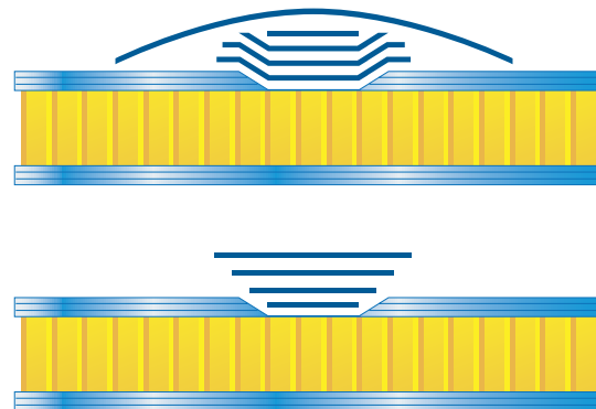
Figure 3-37. Different lay-up techniques.
