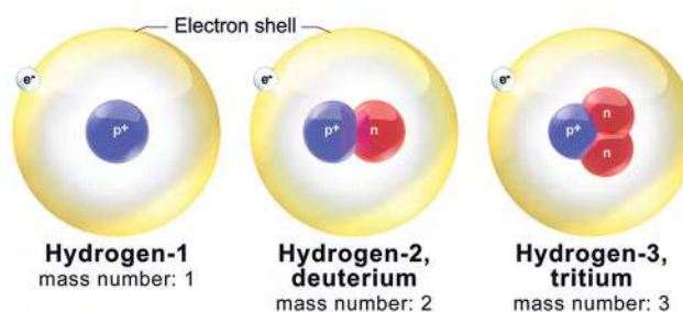
Figure 1-7. Isotopes of hydrogen.
