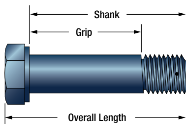
Figure 1-5. Bolt dimensions.
