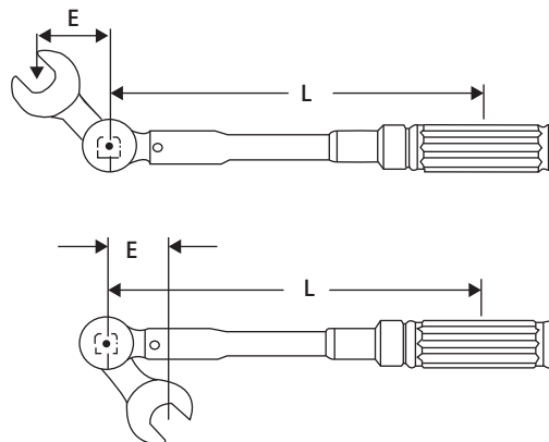
Figure 3-17. Variables for torque formula.
